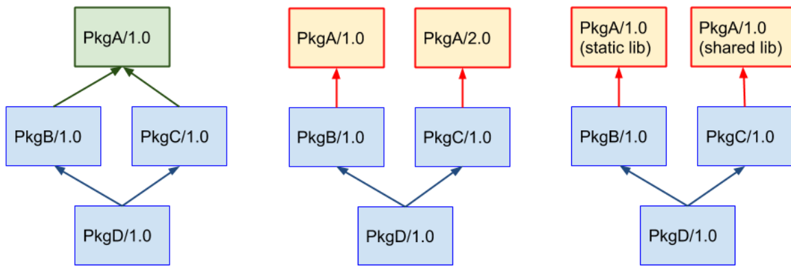
“Diamond” in the dependency graph.
